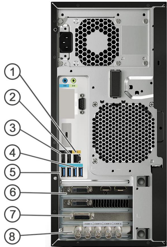
HDV-WSN4SDI Video Core BACK VIEW
